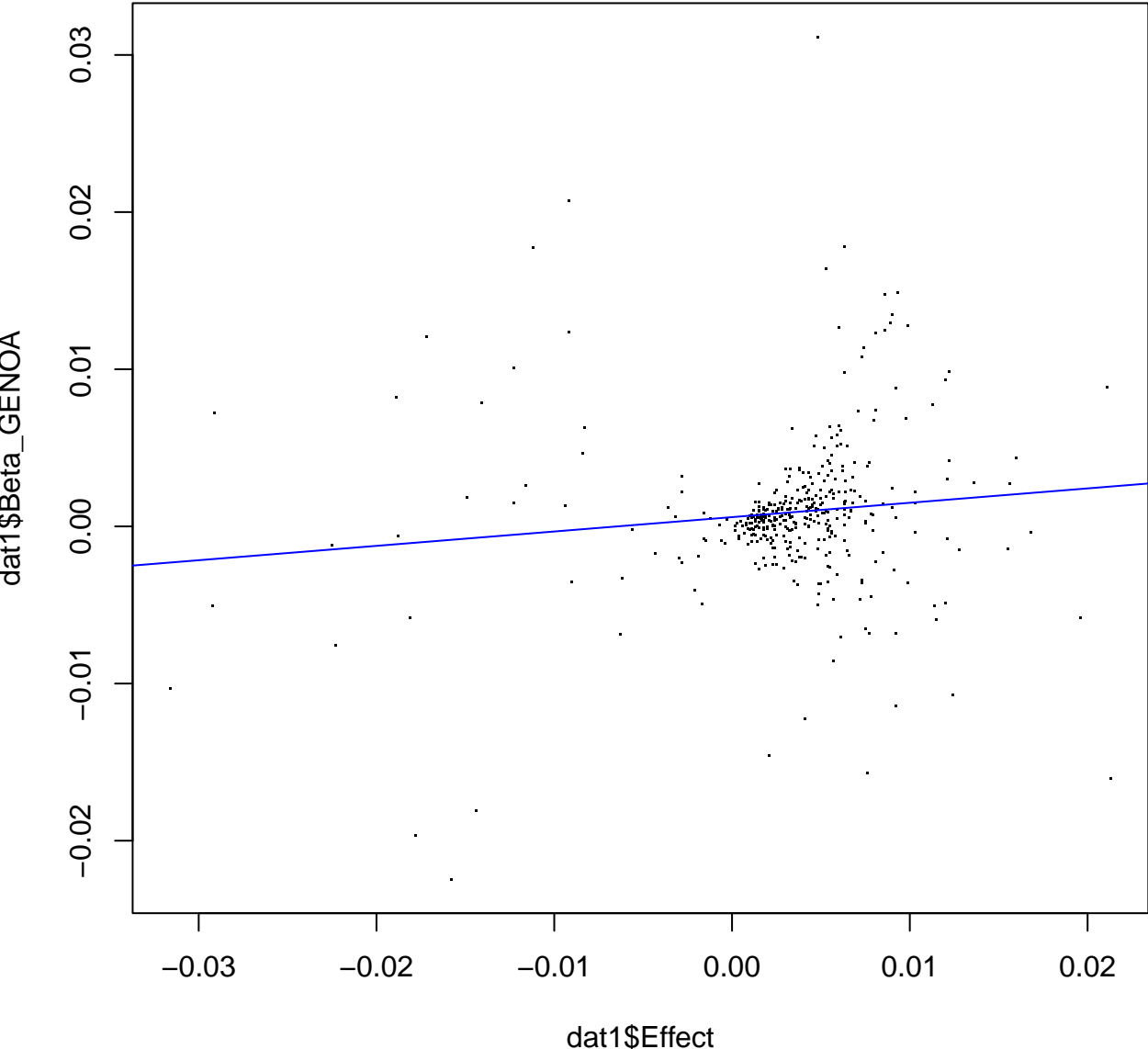
Scatter Plot of Beta Coefficients of EA4 and GENOA (corr=0.116)
